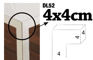
DL52 4x4cm enamelled steel square tubular section 4x4cm from 1m 2 until 1,5m 2 Standard height 73cm
