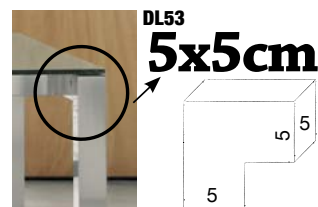
DL53 5x5cm aluminium structure 5x5cm from 0,7m 2 until 2,5m 2 with interior stringers of 10cm to the plan Standard height 73cm
